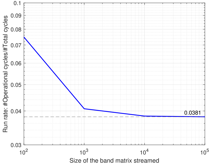
Figure 5.9: Running rate of a RTL kernel’s BMMM operation with MAT_SIZE = 16 and DATA_WIDTH = 8. The running rate has been calculated by dividing the number of working (non-stalled) cycles by the total number of cycles used for the operation.
