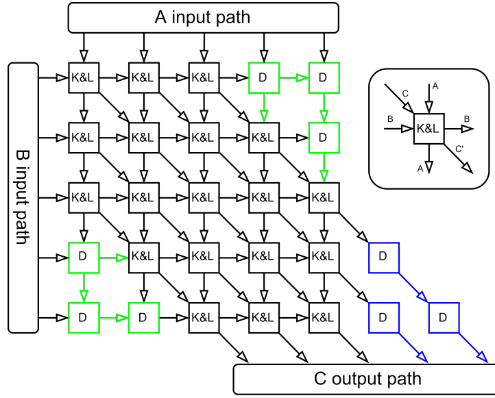
Figure 2.12: Systolic array for GMMM
