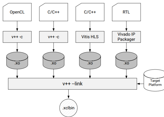
Figure 4.2: Vitis device build process, from [22]
