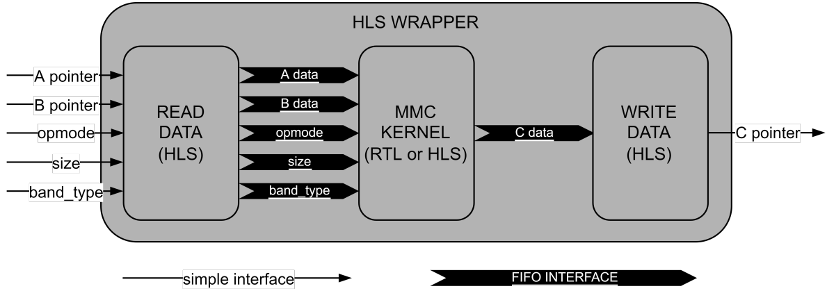
Figure 4.5: Internal structure of the HLS wrapper
