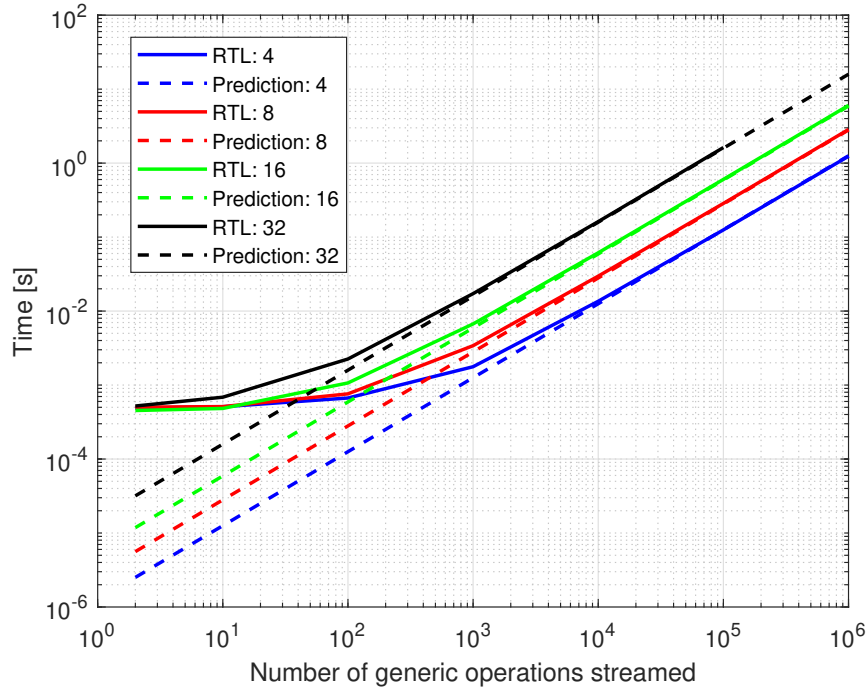
Figure 5.7: Timing results for different amounts of streamed operations for our RTL kernel and the associated theoretical equivalents. Since our HLS and RTL times are so similar, we will only compare with one of them.
