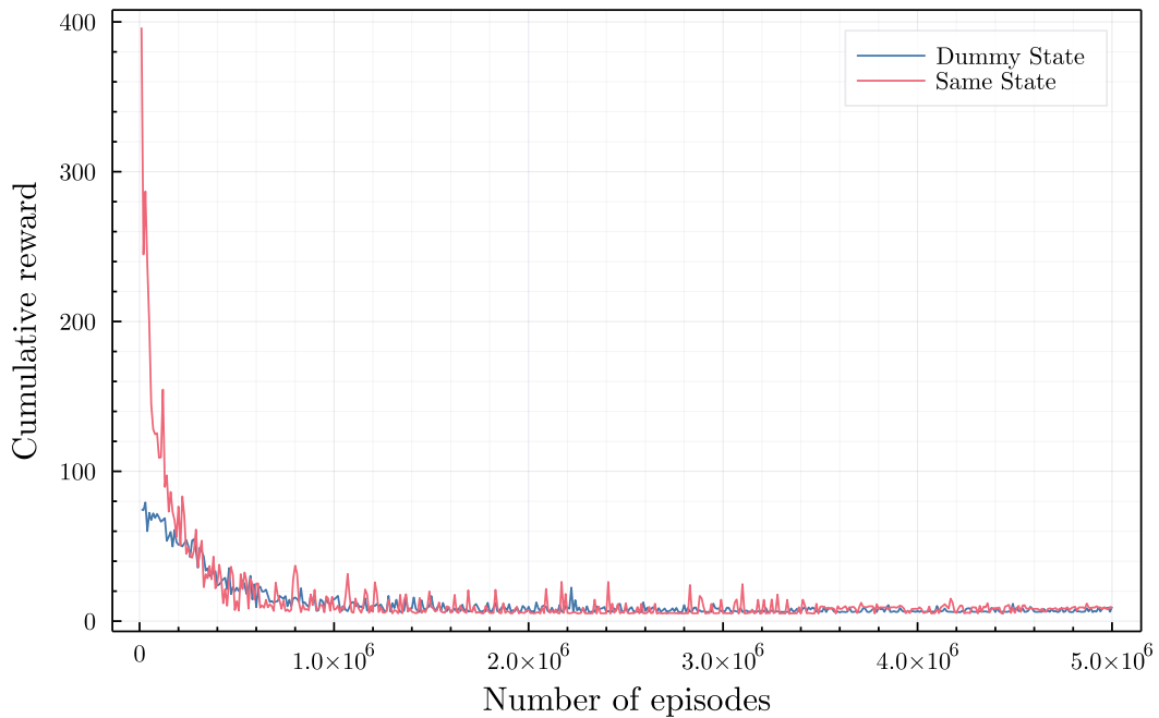
Figure 6.7: Q-Learning for 2 LDs with 100% capacity at the CD and 10 periods using both approaches. Source: Own elaboration.
