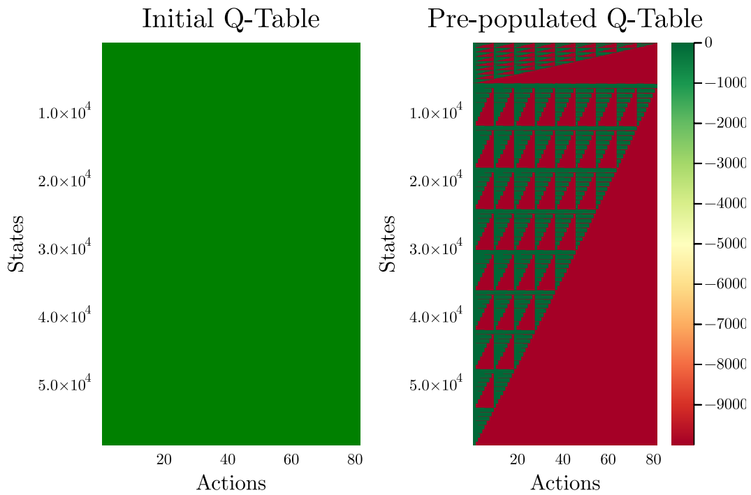
Figure 6.8: Pre-Populated Q-Table for 2 LDs with 100% capacity at the CD and 10 periods.
