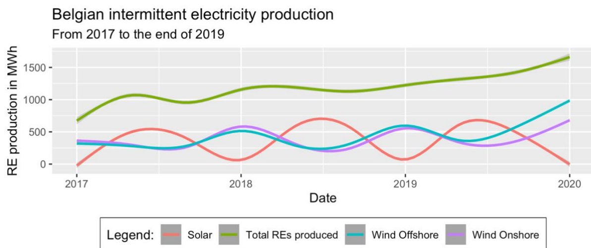
Figure 7 Belgian intermittent electricity production from 2017 to 2019
