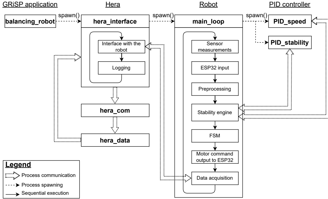
Figure 8.3: Process architecture running on GRiSP.
