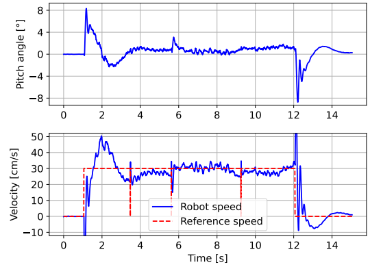
Figure 10.4: Evolution of the angle and velocity of the robot when going forward with an instantaneous velocity profile.
