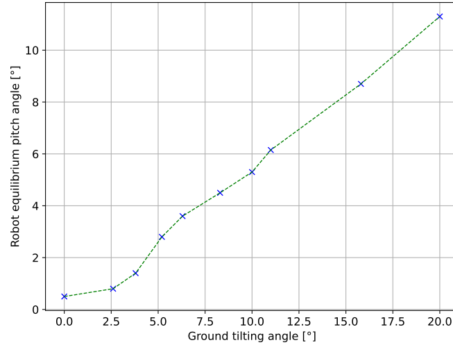
Figure 10.14: Graph showing the equilibrium angle of the robot on a slope.
