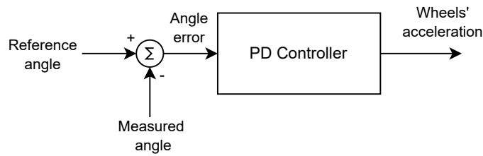
Figure 5.1: PD control system with the error computed from a reference angle set by the user and the measured angle, and return a command for the wheels' accelerations.
