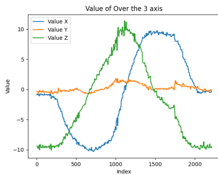
(a) Acceleration values of the 1st gesture
