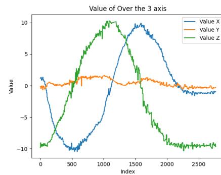
(b) Acceleration values of the 2st gesture
