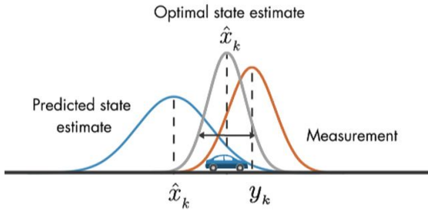
Figure 2.4: Kalman filter illustration[23]
