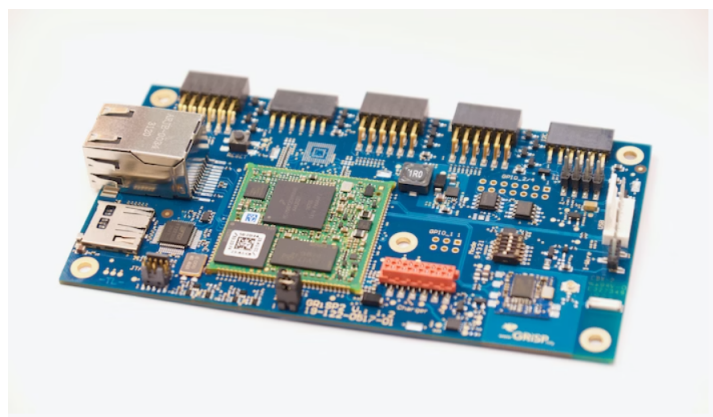
Figure 2.2: Prototype GRiSP2 board
